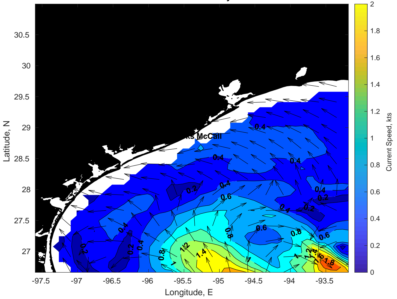
Surface Currents for Brooks McCall at 05-May-2024 00:00:00
